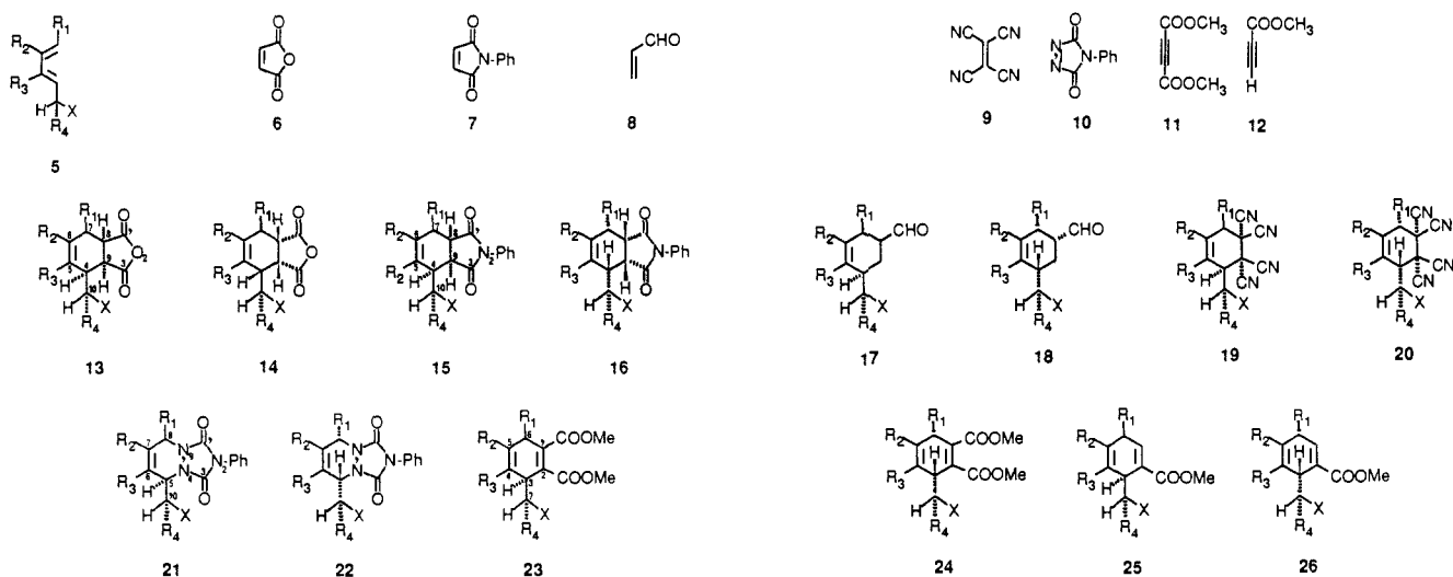
Chart I. Dienes, Dienophiles, and Initial Cycloadducts Listed in Table I a
